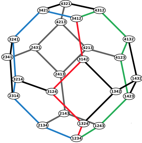
Fig. 9. A permutohedron of order four for a scene with four agents. Three alternative paths implementing the transition from the permutation 1234 to the permutation 3412 are depicted in different colors. Each path consists of a sequence of transitions, each of which can be implemented topologically with a braid generator or its inverse.
