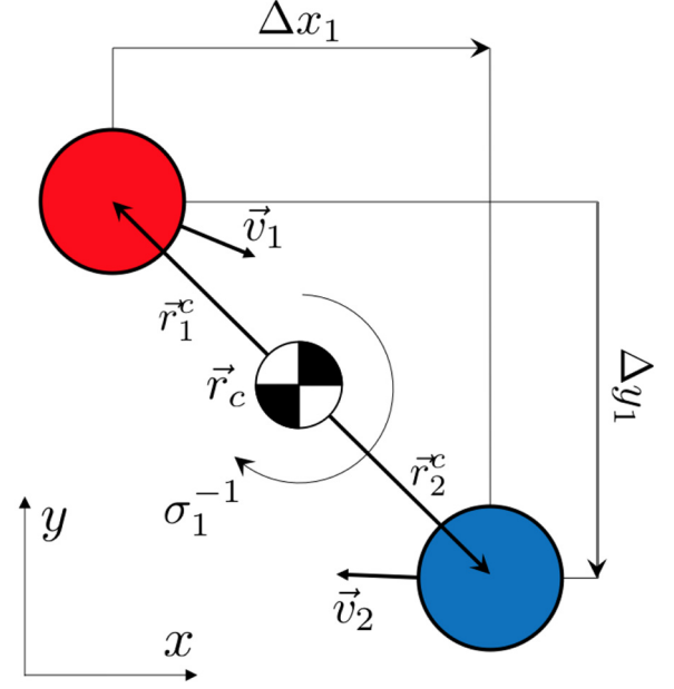
Fig. 7. Demonstration of the momentum heuristic for predicting a generator superscript: the x -projections of the agents' paths are about to cross, forming a \sigma_1^{-1} generator. The z component of their angular momentum is negative, indicating a tendency for a counterclockwise rotation, which indicates a negative braid exponent; likewise, in case the z component of the angular momentum were positive, the emerging exponent would be positive.
